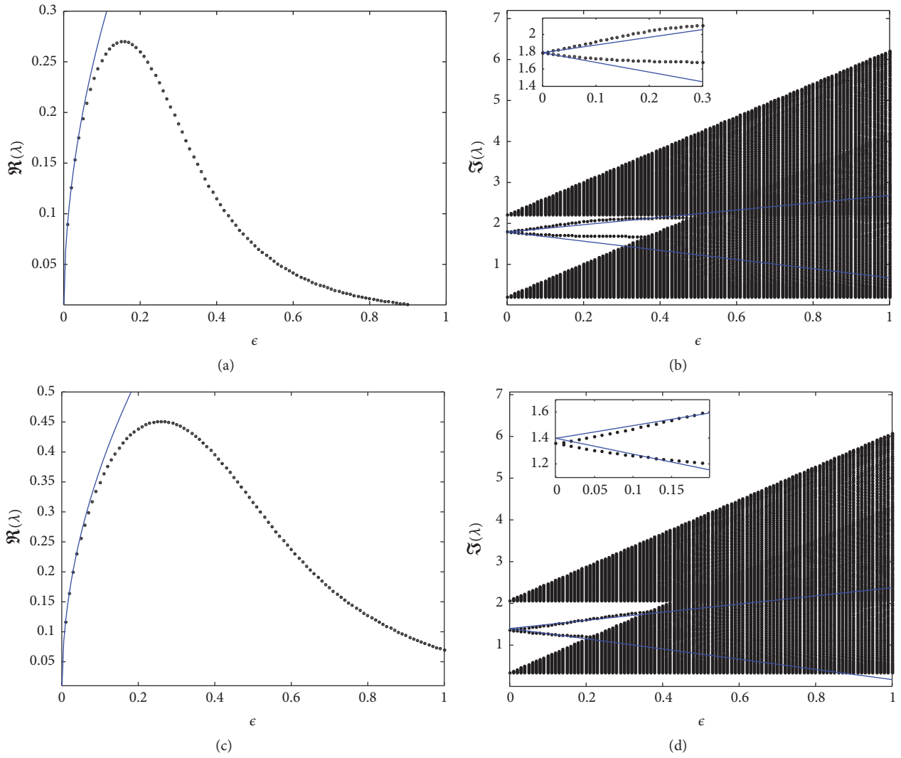
FIGURE 1: Eigenvalues of intersite soliton I with \omega = 1.2 , \gamma = 0 (a, b) and 0.5 (c, d). Dots are from the numerics and solid lines are the asymptotic approximations in Section 4.2.1. The collection of dots forming black regions in the right column corresponds to the continuous spectrum.
