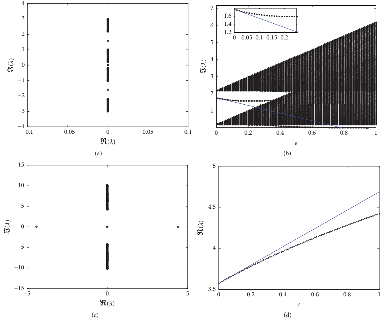
FIGURE 4: (a, c) The spectrum of onsite soliton I in the complex plane for \epsilon = 0.2 . (b, d) The eigenvalue as a function of the coupling and its approximation from Section 4.2.3. (a–d) are for \omega = 1.2 and 5.2 , respectively. Here, \gamma = 0.1 .
