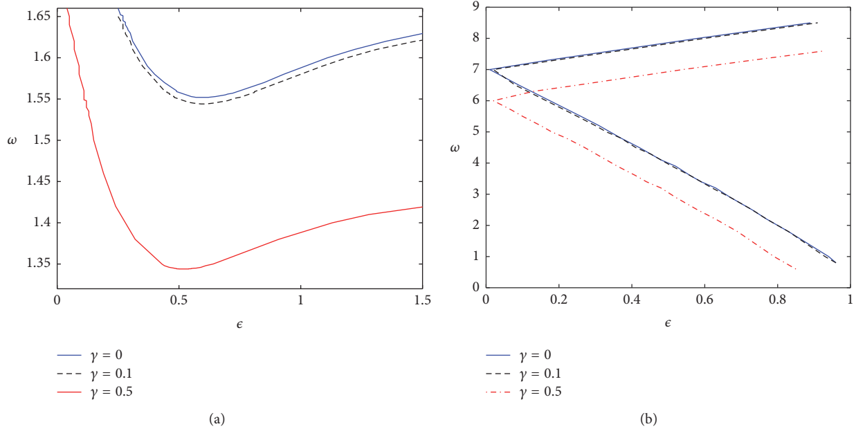
FIGURE 6: The stability region of the onsite soliton type I (a) and II (b) in the (\epsilon, \omega) -plane for several values of \gamma . The solutions are unstable above the curves in panel (a) and between the curves in panel (b).
