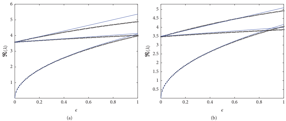
FIGURE 2: The same as in Figure 1 with \gamma = 0 (a) and \gamma = 0.5 (b), but for \omega = 5.2 . In this case, all the eigenvalues are real.
