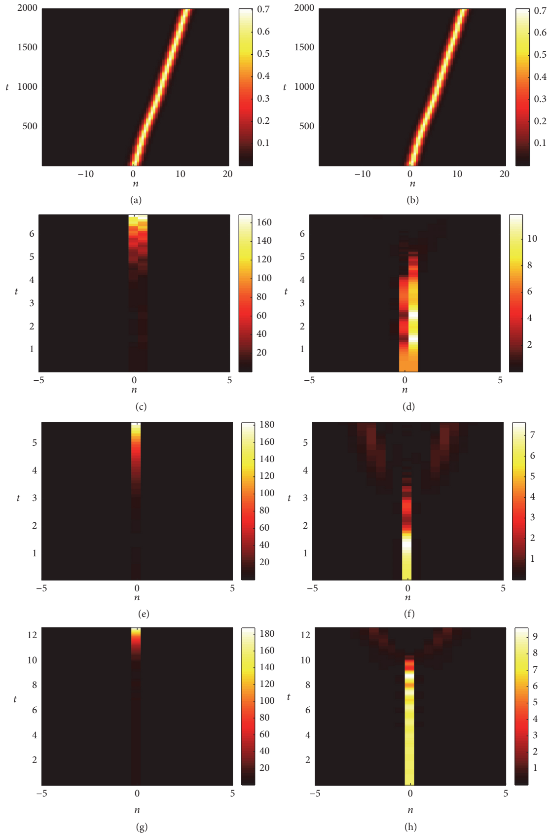
FIGURE 7: The typical dynamics of the instability of the discrete solitons in the previous figures. Here, \gamma = 0.5 and \epsilon = 1 . Depicted in (a–h) are |u_n|^2 and |v_n|^2 , respectively. (a–h) The dynamics of intersite soliton I with \omega = 1.2 , intersite soliton II with \omega = 5.2 , and onsite solitons I and II both with \omega = 5.2 .
