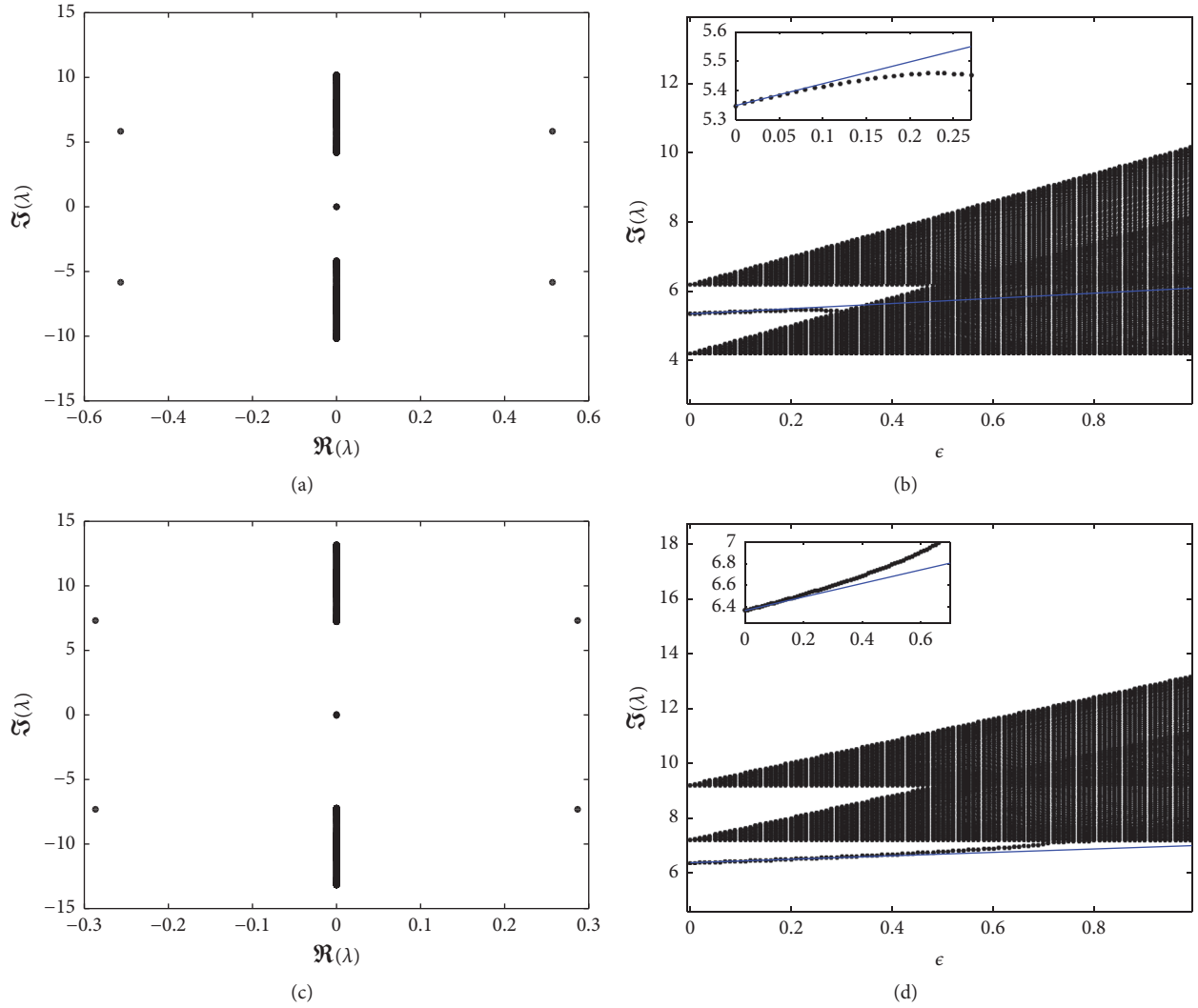
FIGURE 5: The same as in Figure 4, but for onsite soliton II with \omega = 5.2 (a, b) and 8.2 (c, d). (a, c) are with \epsilon = 1 .
