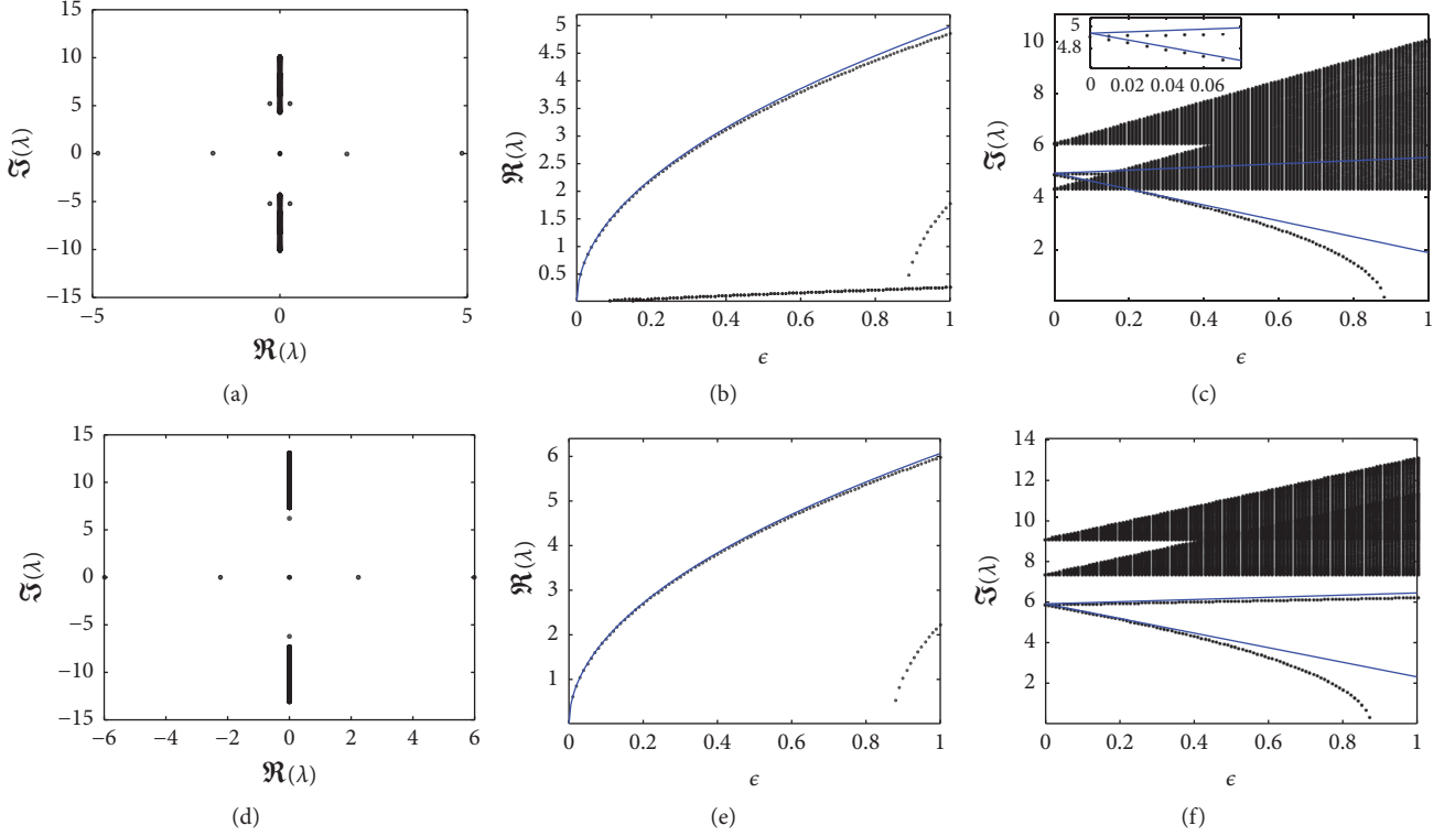
FIGURE 3: The spectra of intersite soliton II with \omega = 5.2 (a, b, c) and 8.2 (d, e, f) and \gamma = 0.5 . The most left panels are the spectra in the complex plane for \epsilon = 1 . (b, c, e, f) The eigenvalues as a function the coupling constant. Solid blue curves are the asymptotic approximations.
