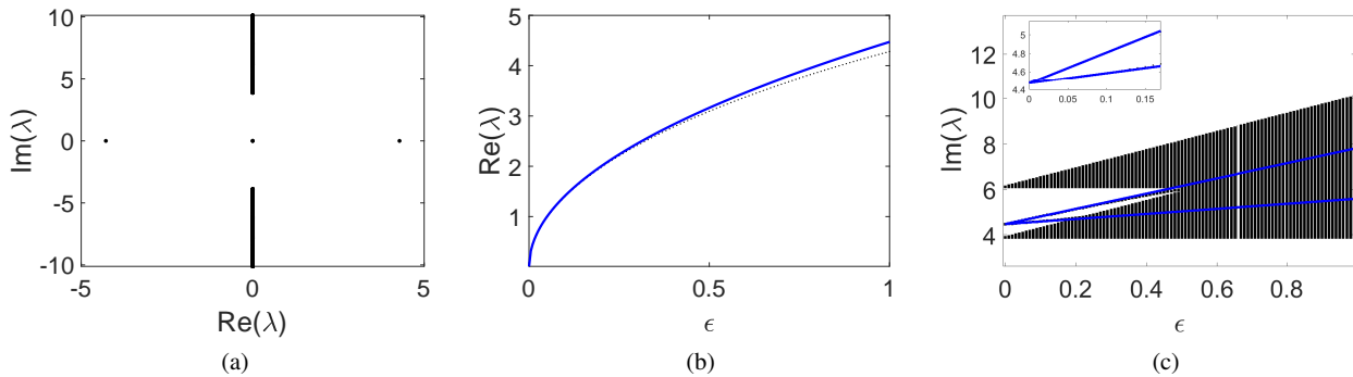
Fig. 3 The spectra of unstable asymmetric intersite discrete solitons with \omega = 5 and \gamma = 0.5 . Panel (a) displays the spectra in the complex plane for \epsilon = 1 . Panels (b) and (c) present the eigenvalues \lambda as a function of the coupling constant \epsilon . The solid blue and dotted curves are attained from the asymptotic approximation and numerical calculation, respectively.
