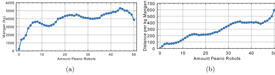
Fig. 9 Analysis of the experimental procedure Diamond, Square, Peano 0-50 increase: (a) collected amount of manganese; (b) relation between the total amount of collected manganese and the distance all agents (robots in the given context) have covered.
