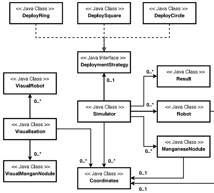
Fig. 3 Conceptual class diagram of the developed application.
