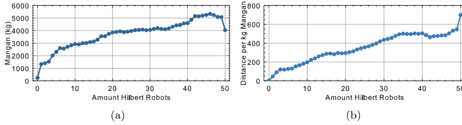
Fig. 11 Analysis of the experimental procedure Diamond, Square, Hilbert 0-50 increase: (a) collected amount of manganese; (b) relation between the total amount of collected manganese and the distance all agents (robots in the given context) have covered.
