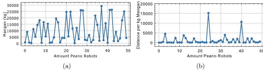
Fig. 15 Analysis of the experimental procedure Lines, Circle, Peano 0-49 increase: (a) collected amount of manganese; (b) relation between the total amount of collected manganese and the distance all agents (robots in the given context) have covered.
