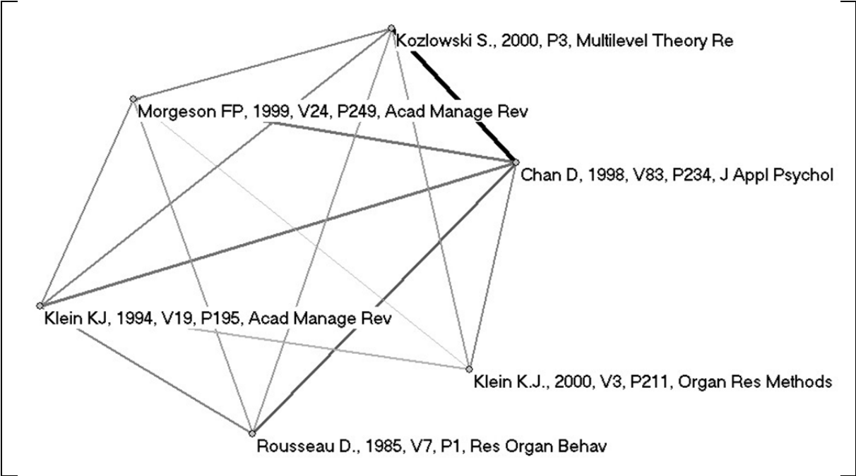
Figure 5: Interrater reliability and agreement
