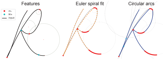
Fig. 3. Feature extraction (left) followed by Euler spiral fitting (middle) and arc decomposition (right) of a sample from the UIJ handwritten character dataset. The arcs in red indicate regions with approximately constant curvature corresponding with curvature extrema.
