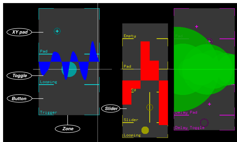
Figure 4. Stage 3: Example of AVUI built with the toolkit, using three zones, with different UI elements and visualizations (explanatory labels in white).
