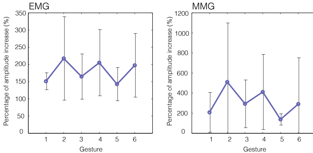
Fig. 11. Percentage of amplitude increase between the condition “more power” and the baseline. On the left are reported the percentages related to EMG, on the right those related to MMG.
