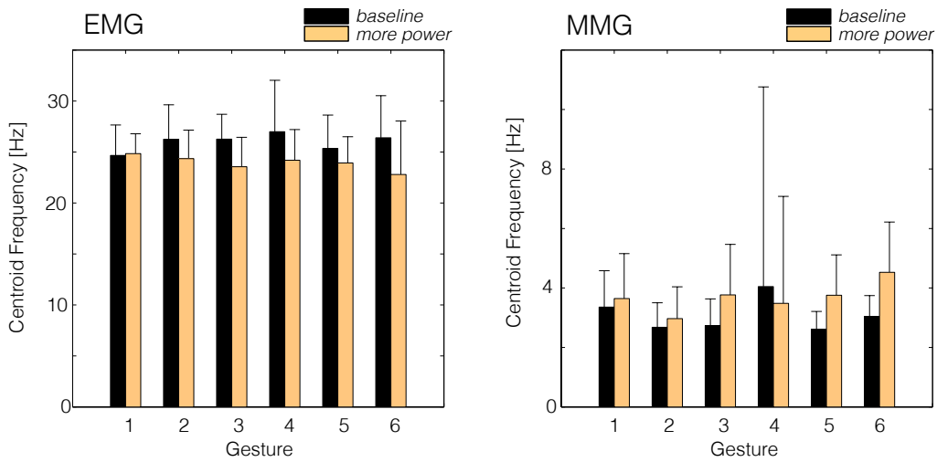
Fig. 9. Centroids for both EMG (left) and MMG (right) averaged across participants and trials. Black bars show the mean centroid frequency when no variation is applied (baseline), orange bars report mean centroid frequency when more power is exerted.
