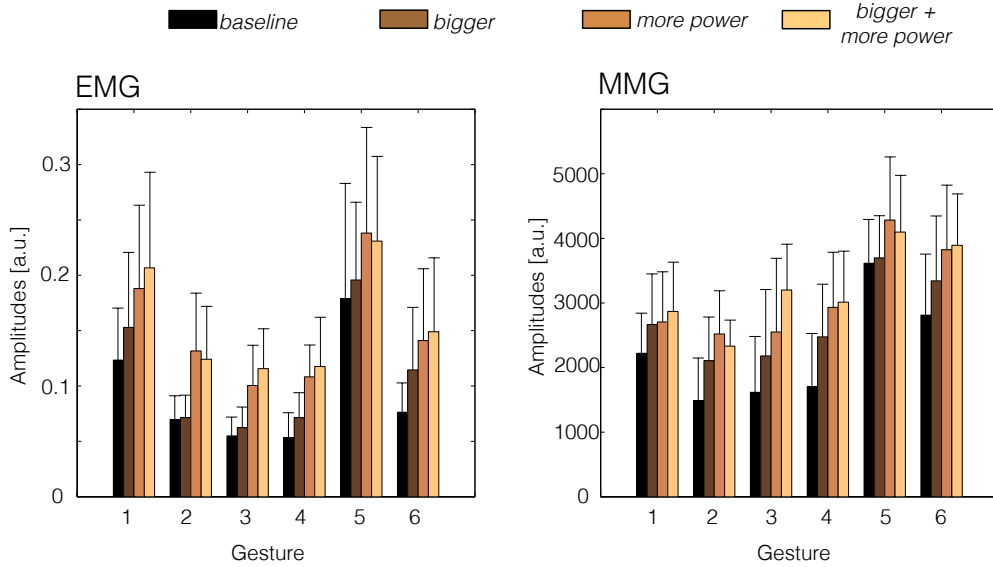
Fig. 13. Amplitudes for both EMG (left) and MMG (right) averaged across participants and trials. Four conditions are considered: baseline, bigger, more power and bigger+more power.
