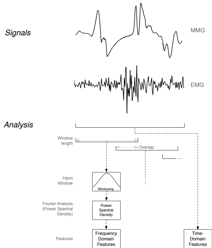
Fig. 4. The feature extraction dataflow.
