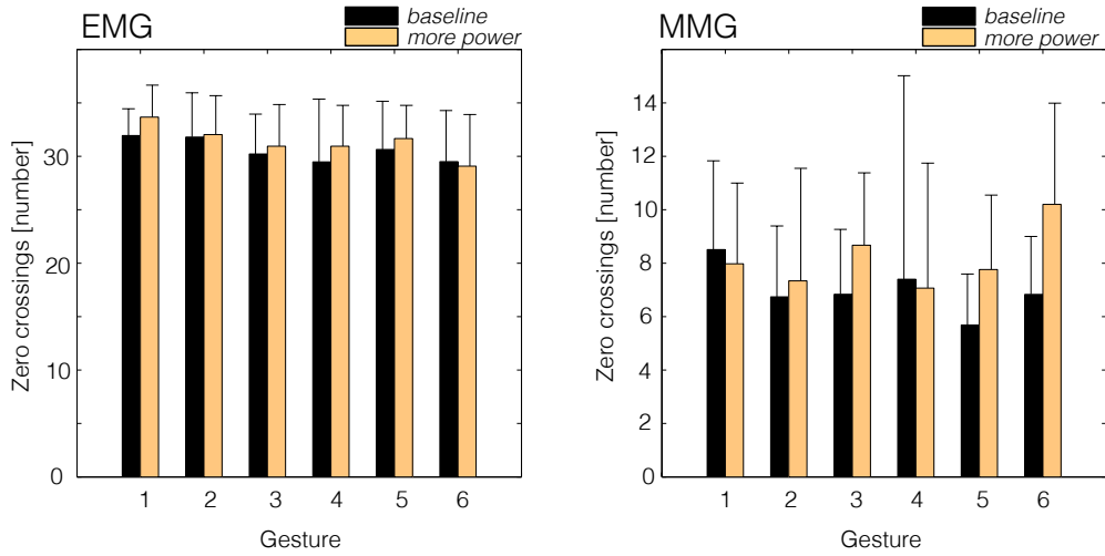
Fig. 8. Zero crossings for both EMG (left) and MMG (right) averaged across participants and trials. Black bars show the mean number of zero crossings when no variation is applied (baseline), orange bars report mean number of zero crossings when more power is exerted.
